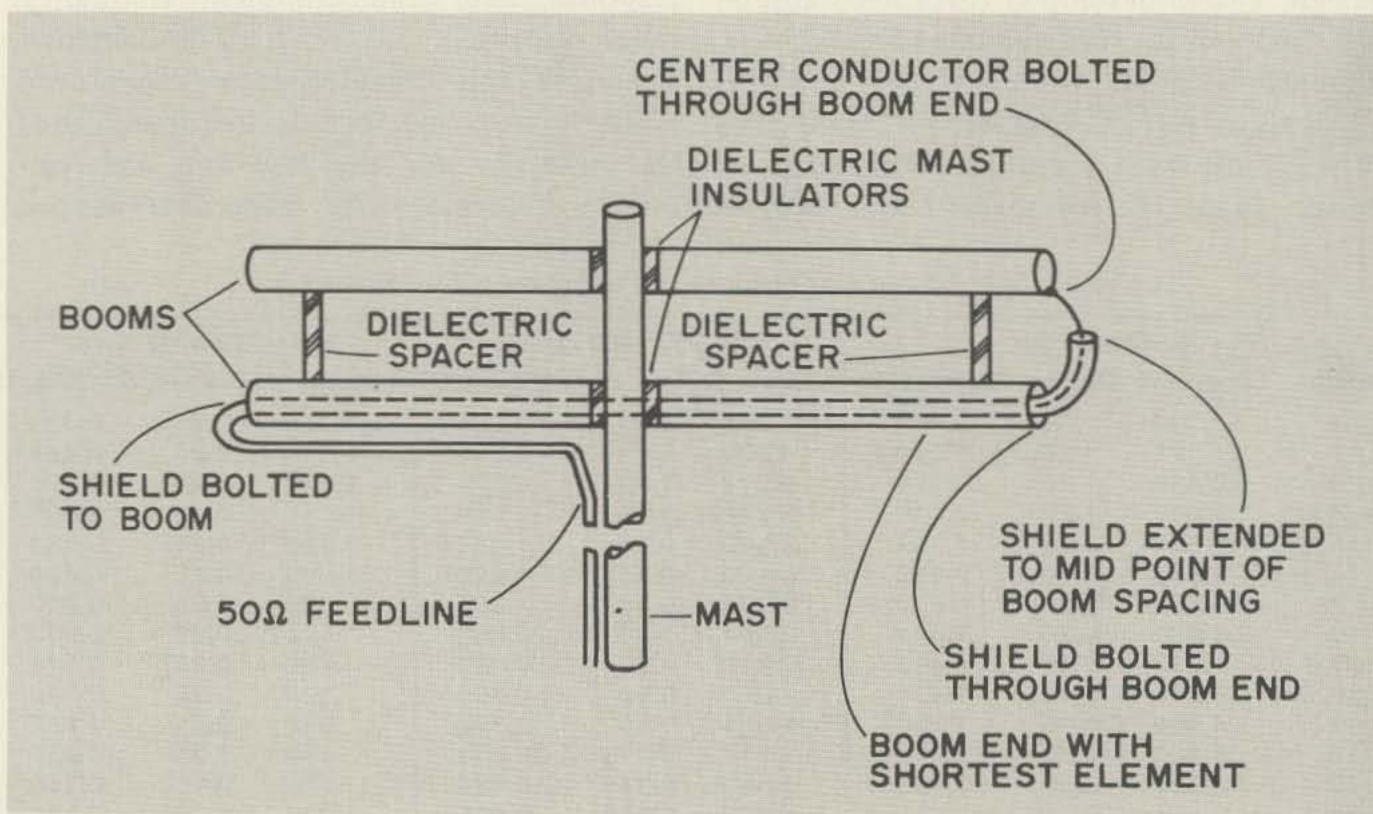
Fig. 2. Feeding the log periodic is relatively simple. Just remove the outer plastic jacket from feedline for the entire length of the boom, so that the coax shield is permitted to short itself inside the boom as well as the solid electrical connections at each end of the boom.
